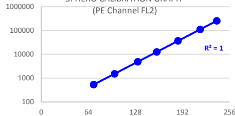
SPHERO CALIBRATION GRAPH (PE Channel FL2)
